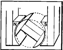
Fig. 2—Position of the armature between the magnets of the magneto, showing direction of rotation
